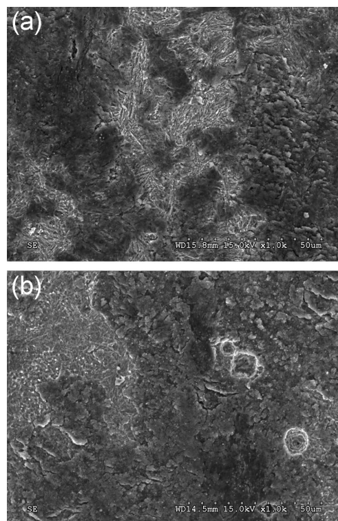
Fig. 8. Surface appearance of 67SiMnCr6-6-4 bearing steel after austempering (a) and quenching and tempering (b) after corrosion tests in Na 2 SO 4 neutral environment
