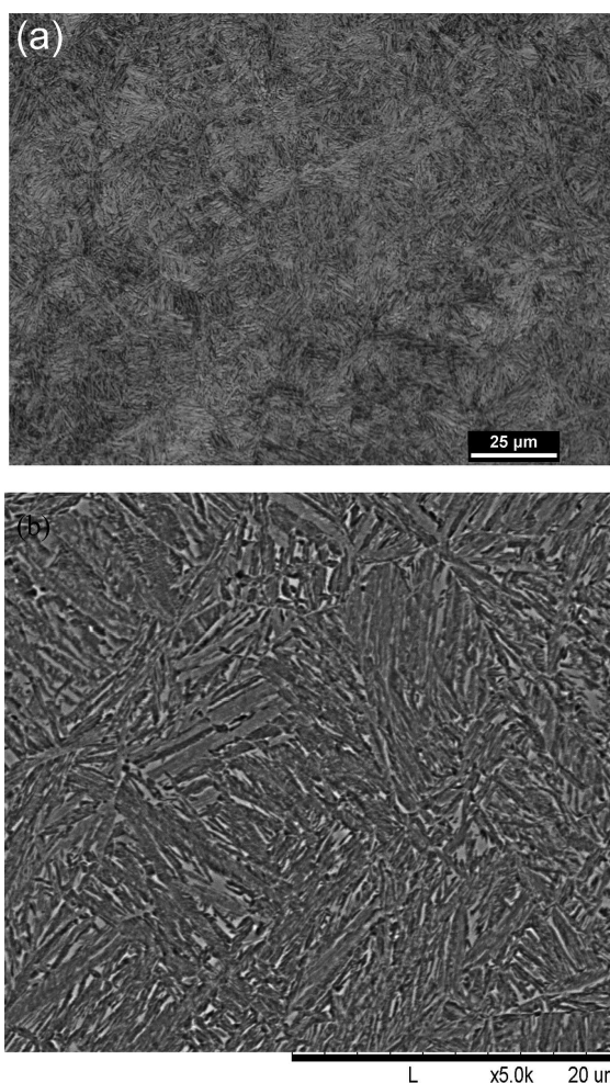
Fig. 1. Microstructure of 67SiMnCr6-6-4 bearing steel after austempering treatment at 240°C for 61h observed using light microscope (a) and scanning electron microscope (b)
