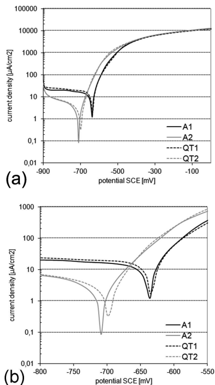
Fig. 7. Polarization curves obtained for 67SiMnCr6-6-4 bearing steel after various heat treatments in Na 2 SO 4 neutral environment (b - magnification of the corrosion potential area)
