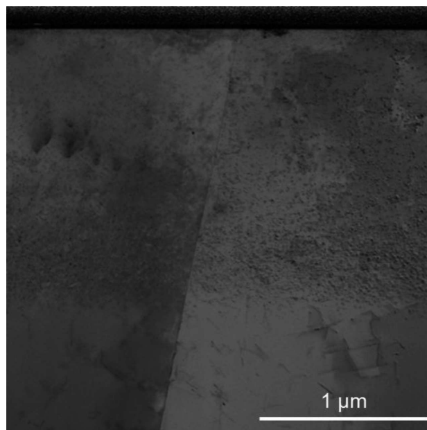
Fig. 3. Cross-sectional micrograph of the irradiated sample
