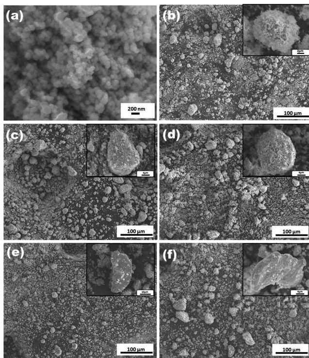
Fig. 2. Morphology of the nano Al-powders by high energy ball milling with the milling time. SEM micrographs of (a) 0 min, (b) 10 min, (c) 30 min, (d) 1 h, (e) 2 h and (f) 3 h. (inset: high magnified SEM images)
