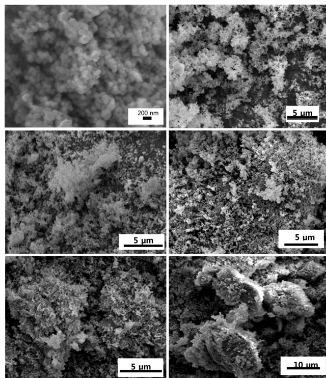
Fig. 1. Morphology of the nano Al-powders by low energy ball milling with the milling time. SEM micrographs of (a) 0 min, (b) 10 min, (c) 30min, (d) 1h, (e) 5 h and (f) 30 h. ( inset: high magnified SEM images)
