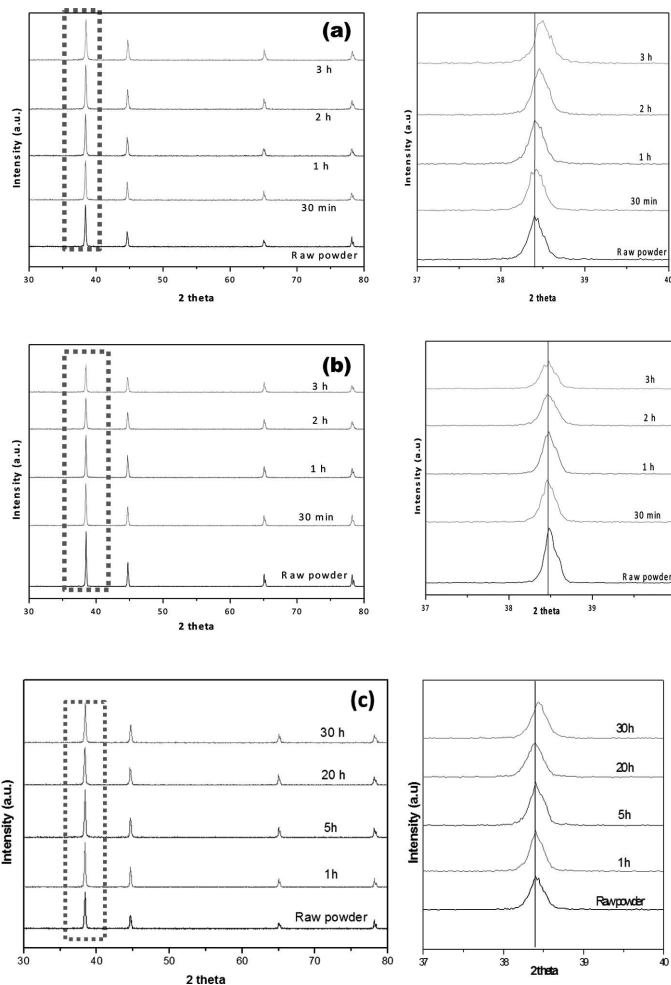
Fig. 4. XRD analysis of (a) nano Al-powders (b) micron Al-powders by high energy ball milling, and (C) nano Al-powders by low energy ball milling
