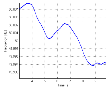
Fig. 15. Recorded frequency fluctuations of real life power waveforms – example 1.
