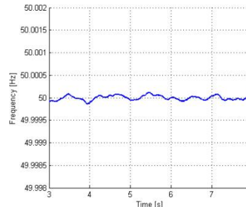
Fig. 11. Recorded frequency fluctuations of simulated signal with white noise, (fundamental harmonics f=50 Hz, estimated precision 3\sigma = 153.0 \mu\text{Hz} ).
