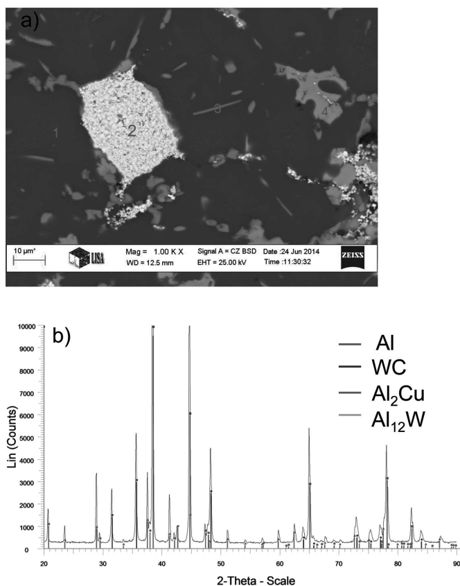
Fig. 5. a) Microstructure (1=Al, 2=WC, 3=Al 2 Cu, 4=Al 12 W) and b) XRD pattern of Al 15 WC-30 composite
