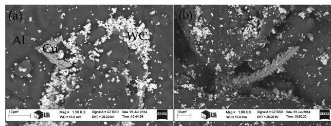
Fig. 1. SEM micrographs of the Al15WC-30 composite powder in a) 1500x b) 1000x magnification
