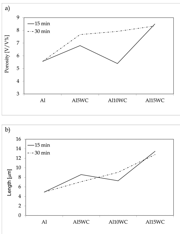
Fig. 4. a) Amount and b) mean size of the pores
