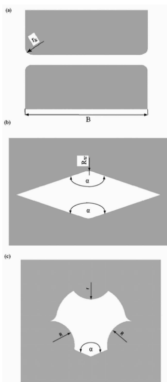
Fig. 2. Shape of anvils: (a) – flat ( r_k = 0.10B ), (b) – radial-rhombic with an impression angle of \alpha = 135^{\circ}/135^{\circ} ( R_w = 0.35D_0 ), (c) – special tri-radial ( R/D_0 = 0.40 , r/D_0 = 0.35 and \alpha = 135^{\circ} )
