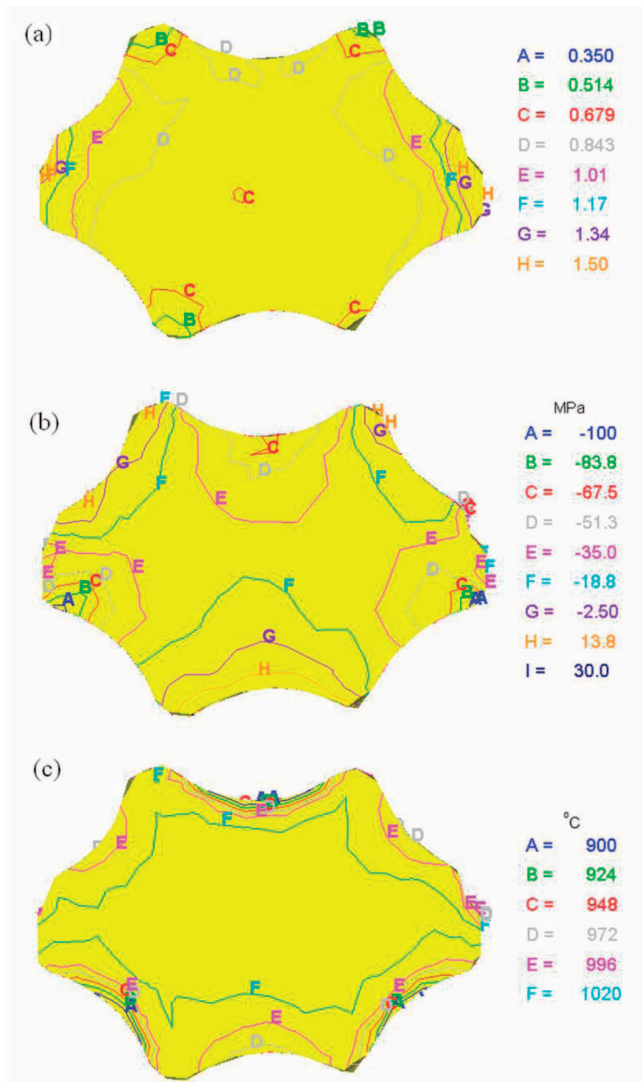
Fig. 5. Distribution of effective strain (a), mean stress (b) and temperature (c) on the specimen cross-sectional surface after cogging process in special tri-radial anvils. True strain \varepsilon_h = 0.70
