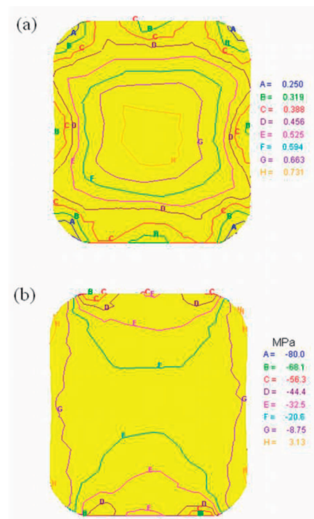
Fig. 3. Distribution of effective strain (a) and mean stress (b) on the specimen cross-sectional surface during cogging process in flat anvils after the second reduction ( \varepsilon_h = 0.70 )
