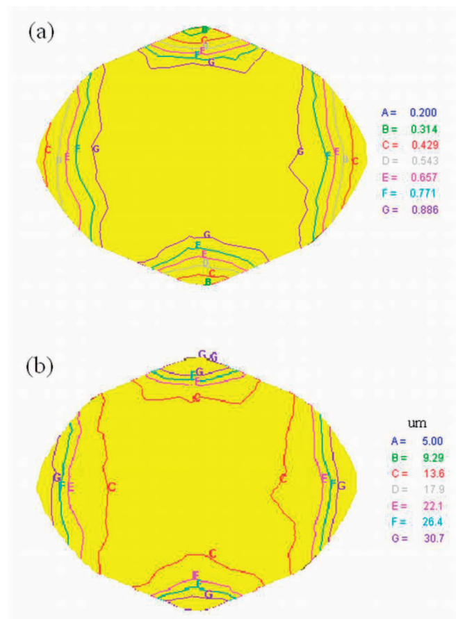
Fig. 7. Distribution of the dynamically recrystallized volume fraction (a) and mean grain size (b) on the specimen cross-sectional surface after cogging process in radial-rhombic anvils with an impression angle of \alpha = 135^\circ/135^\circ . True strain \varepsilon_h = 0.70
