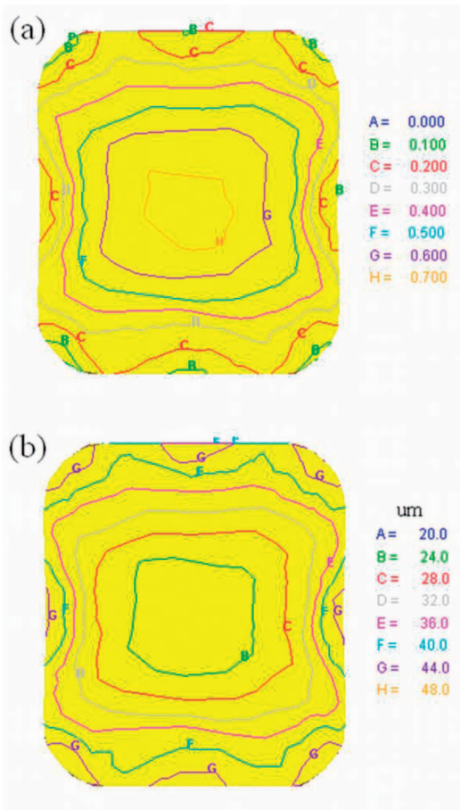
Fig. 6. Distribution of the dynamically recrystallized volume fraction (a) and mean grain size (b) on the specimen cross-sectional surface after cogging process in flat anvils. True strain \varepsilon_h = 0.70
