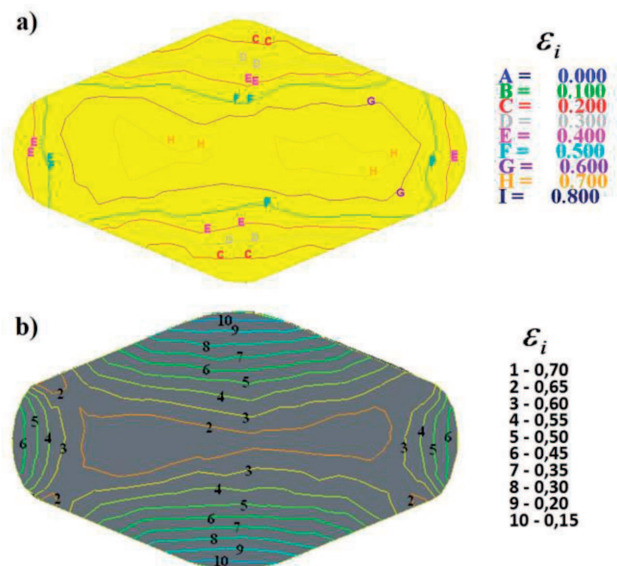
Fig. 9. Comparison of the theoretical (a) and experimental (b) effective strain ( \epsilon_i ) distribution on the cross-sectional surfaces of Ti-6Al-4V alloy specimens deformed in radial-rhombic anvils with an impression angle of \alpha = 135^\circ/135^\circ . Relative feed l_w = 0.75 , true strain \epsilon_h = 0.35
