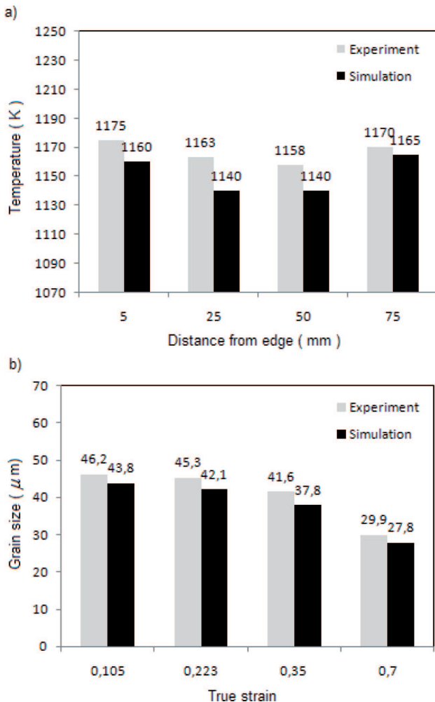
Fig. 10. Comparisons between the experimental and simulated results after cogging process in special tri-radial anvils: (a) temperature of the longitudinal section ( l_w = 0,75 ; \varepsilon_h = 0,70 ), (b) average grain sizes in the centre of the specimens deformed at different true strain
