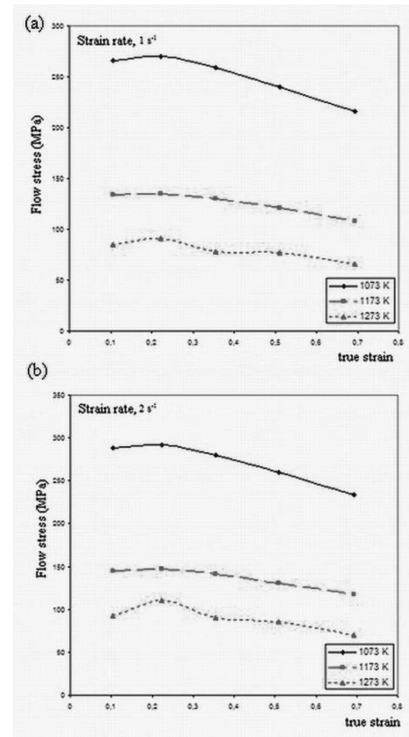
Fig. 1. Variation of flow stress for the Ti-6Al-4V alloy as a function of true plastic strain and temperature, for different strain rate values, i.e.: (a) – \dot{\varepsilon} = 1s^{-1} and (b) – \dot{\varepsilon} = 2s^{-1}
