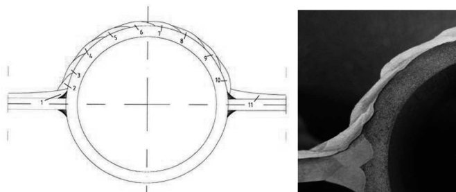
Fig. 7. Single-pass surfacing
