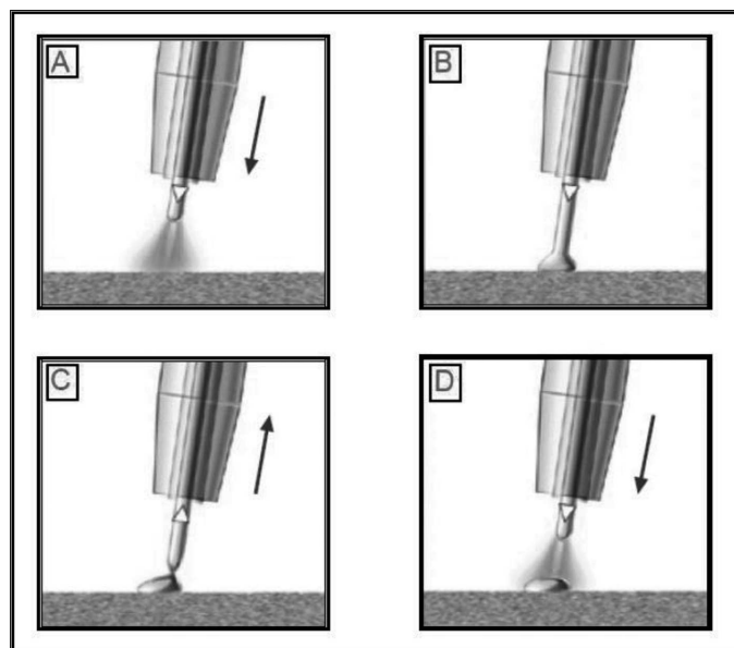
Fig. 6. A process of CMT method of surfacing by welding Source: www.fronius.com
