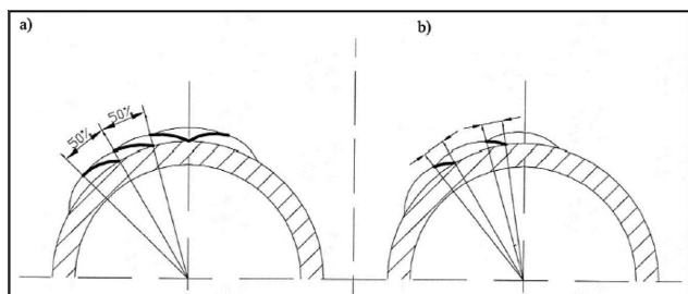
Fig. 9. Single-pass surfacing – overlapping beads
