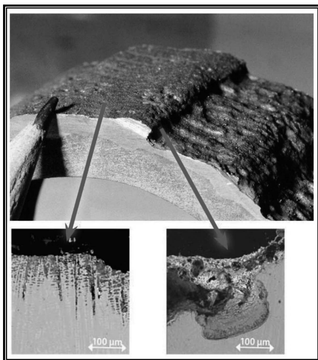
Fig. 13. Comparison of high-temperature corrosion occurring alongside dendrites and pits as a result of melted chlorines [11]
