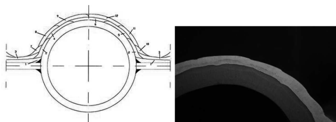
Fig. 8. Two-pass surfacing
