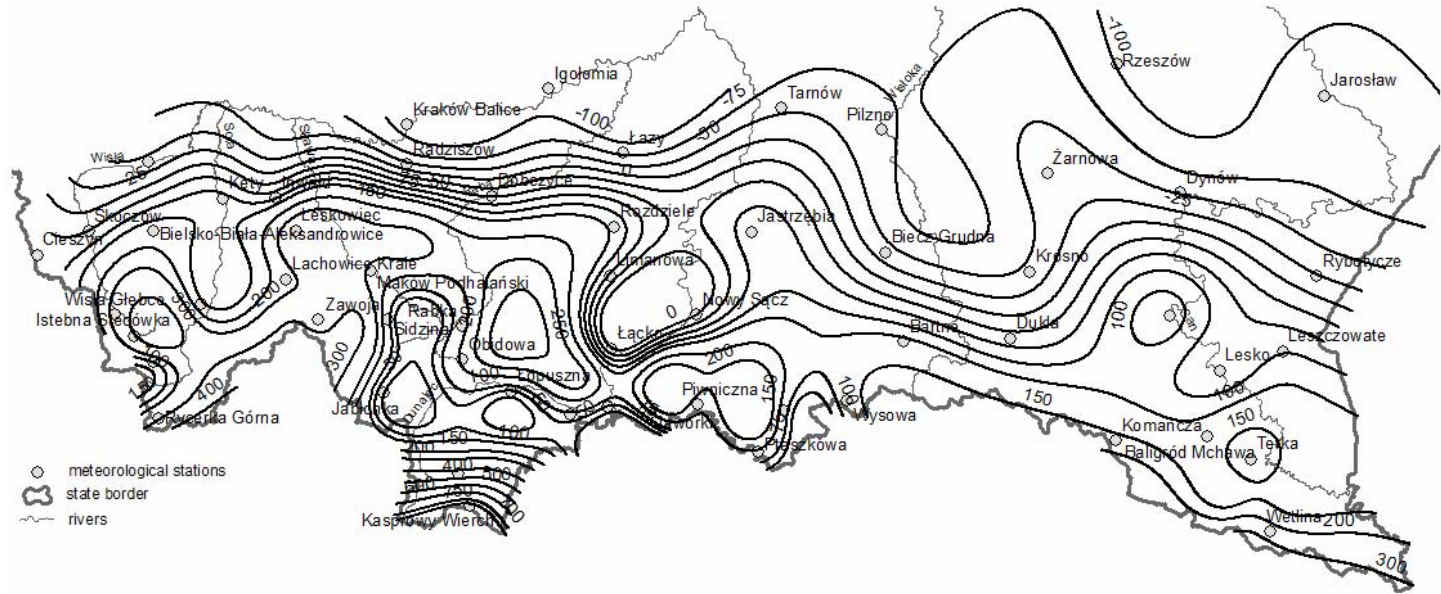
Fig. 3. Map of the Polish Carpathian showing isolines of average climatic water balance ( P - ET_o , mm) – water surplus and deficit – during the period May–October from 1990 to 2005
