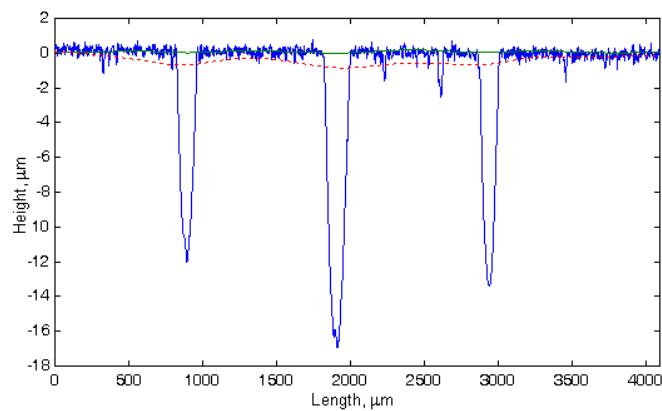
Fig. 9. Unfiltered profile (thick line) with burnished oil pockets and waviness profiles after using a robust filter (dashed line) and a modified robust filter (thin line).
