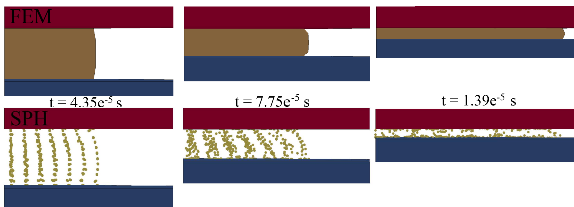
Fig. 7. Copper shaper deformation comparison for both cases.
