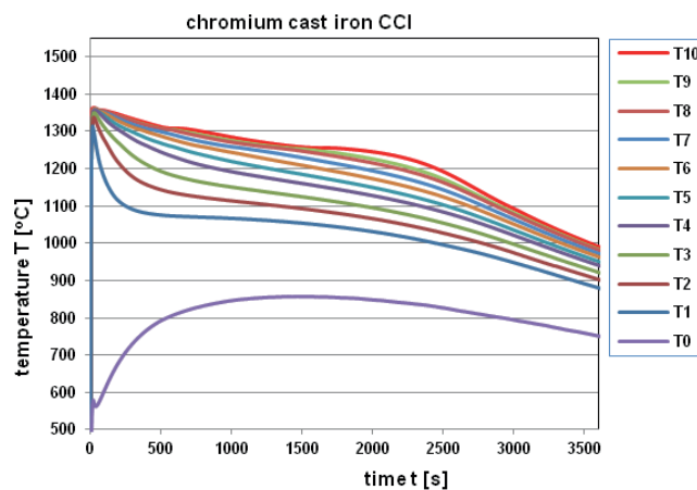
Fig. 3. The cooling curves of studied chromium cast iron CCI
