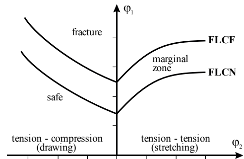
Fig. 1 Forming Limit Diagram
