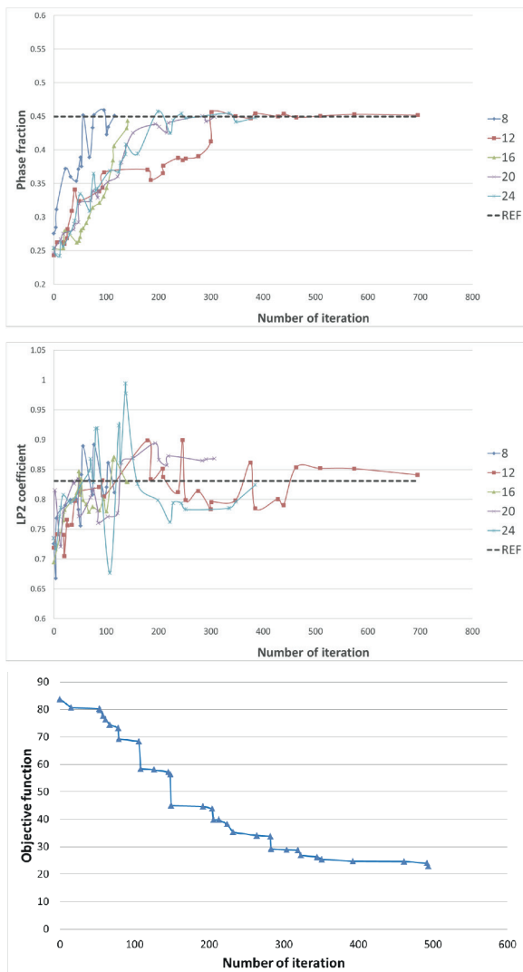
Fig. 8. Convergence of optimization procedure for two coefficients (for different number of NURBS control points) and objective function (12 NURBS control points)
