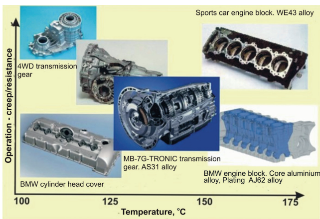
Fig. 1. Working temperature and application of magnesium alloy elements in the automotive industry [5]
