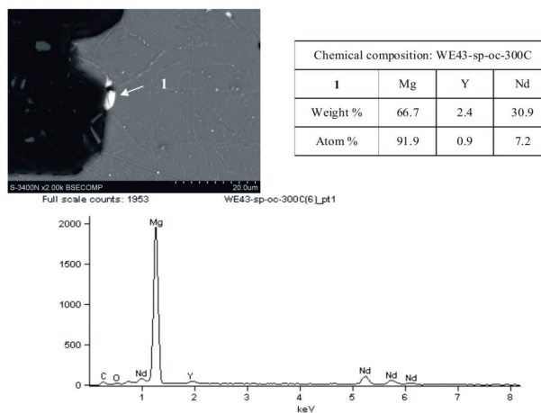
Fig. 9. Results of chemical microanalysis of phase on the surface of the WE43-T6 alloy joint fracture after the tensile test at the temperature of 300°C
