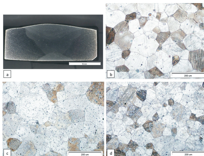
Fig. 4. Research material - welded joint of the WE43 alloy after solution heat treatment (8 h/525°C/air) and ageing (16 h/250°C/air): a) macrostructure of the joint, b) microstructure of the base material, c) growth of the grain in the heat affected zone, d) grain refinement in the area of the weld
