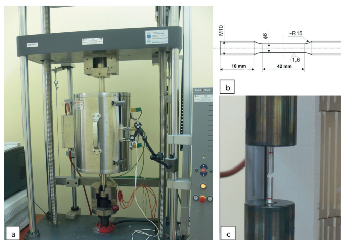
Fig. 5. Tensile test: a) Kappa 50 DS tensile-testing machine, b) sample for tensile tests, c) view of the tensile-testing machine chamber with a broken sample
