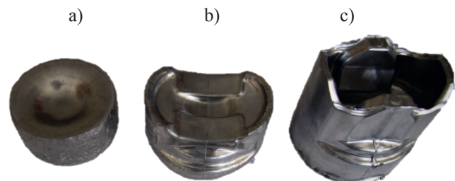
Fig. 22. Forging shapes after operations of: a) flattening, b) initial forging and c) finishing forging of a lead piston
