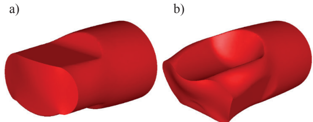
Fig. 9. Shapes of the forgings after flattening: a) before changes and b) after tool shape optimization
