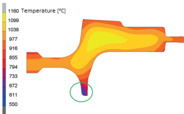
Fig. 24. Temperature distribution in the cross section of a flange-type forging with the marked area of cooling after die forging
