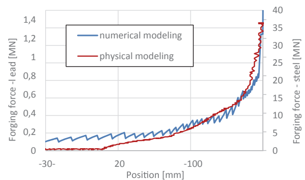
Fig. 23. Comparison of the forming force courses obtained from the physical and numerical modeling
