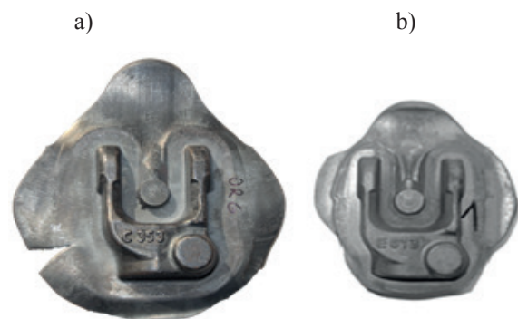
Fig. 10. Comparison of the forging shape: a) before tool modification and b) after tool modification [8]
