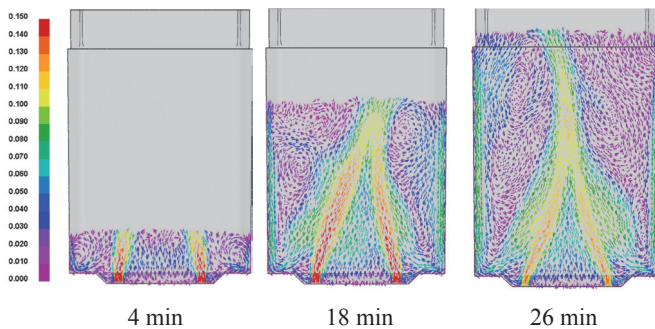
Fig. 3. The character of the steel flow during the bottom filling of the slab mould using velocity vectors in \text{m}\cdot\text{s}^{-1}
