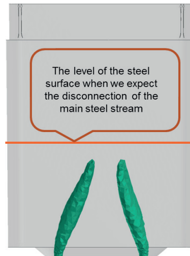
Fig. 4. The velocity limit 0.1 \text{ m}\cdot\text{s}^{-1} displays using the cut-off function
