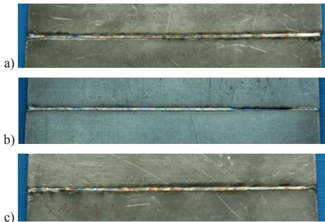
Fig. 8. A view of the weld root (bottom) of the test joints of 0.8 mm thick electro-galvanized steel sheet DC04, autogenously welded by a disk laser (Table 4); a) J1, b) J2, c) J3
