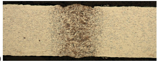
Fig. 6. Cross sections of the bead-on-plate welds produced on the 0.8 mm thick electro-galvanized steel sheet DC04 by a disk laser at very similar heat input, Table 3; a) bead B4 (750 W, 2.0 m/min, 22.5 J/mm), b) bead B8 (2000 W, 6.0 m/min, 20 J/mm)
