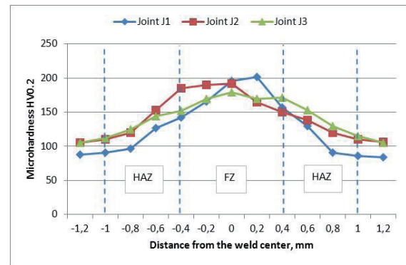
Fig. 11. Microhardness distribution (profile) across the butt joints of 0.8 mm thick electro-galvanized steel sheet DC04, welded by a disk laser (Table 4)
