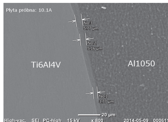
Fig. 8. Microstructure and bond characteristic of sample plate number 10.1A
