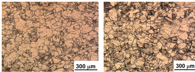
c) sample after the 4 th pass d) sample after the 6 th pass
