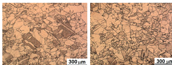
a) sample of initial state
