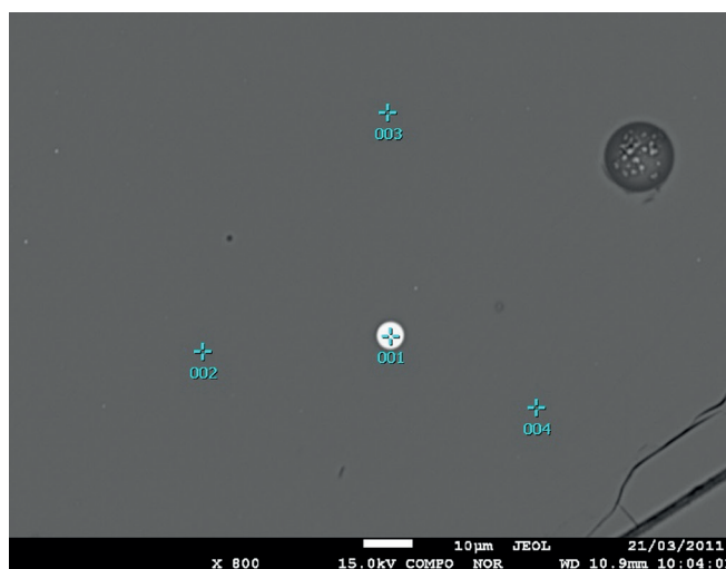
Fig. 2. Hyaline microstructure; microphotography from X-ray spectral microanalysis, blast furnace slag
