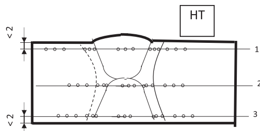
Fig. 17. A way of doing a hardness test [19]
