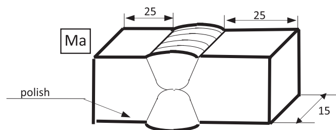
Fig. 14. A way of preparing a metallographic specimen [10]
