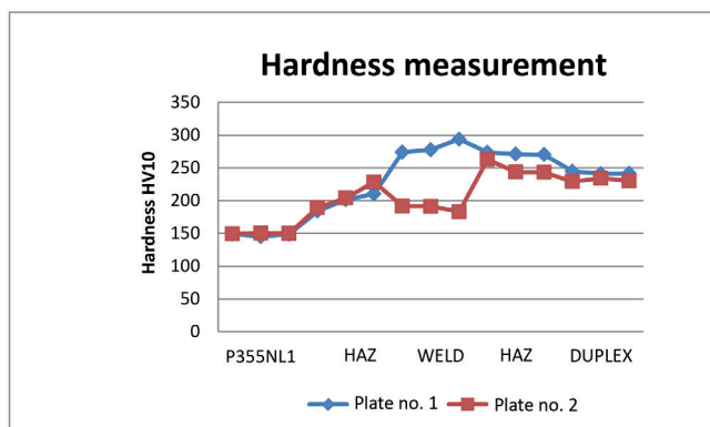
Fig. 18. Results of the hardness measurement
