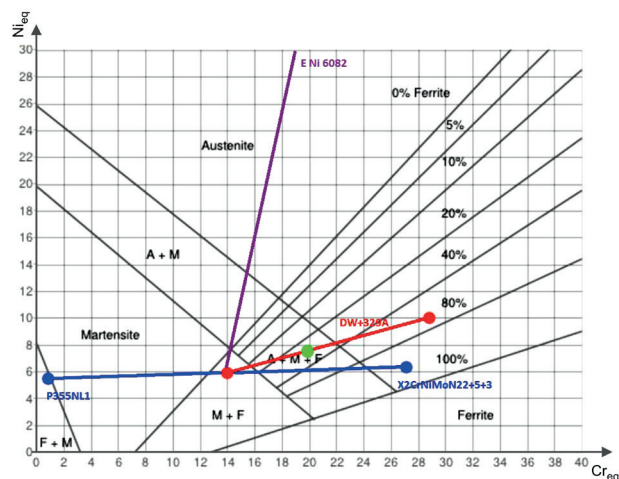
Fig. 1 The Schaeffler's diagram [17]
