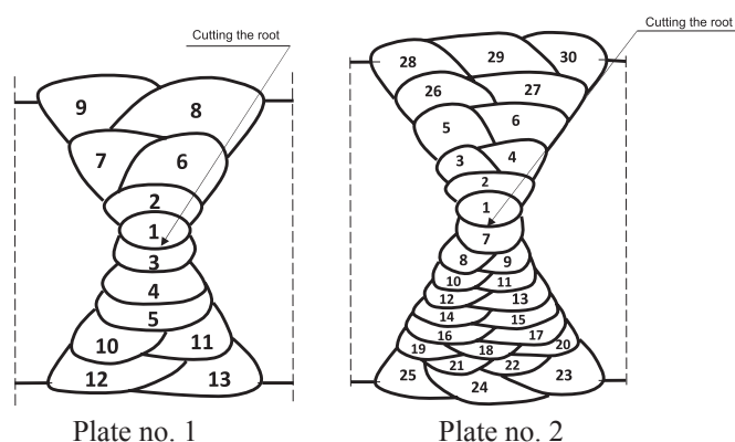
Fig. 2. An order of applying beads
