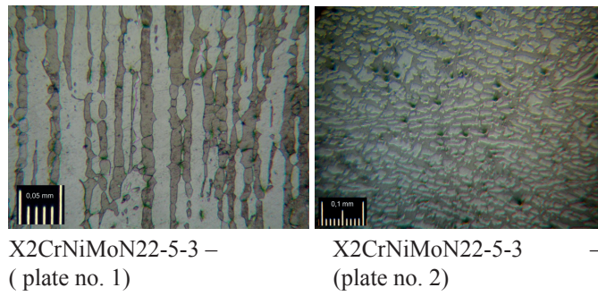
Fig. 16. Microscopic pictures of plates
