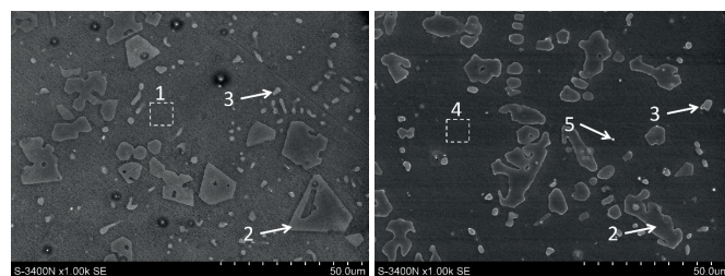
Fig. 5. SEM image of solution-treated Mg-5Si-7Sn alloy (a) and Mg-5Si-7Sn-2Al alloy (b) and EDS results from points marked in the Figures
