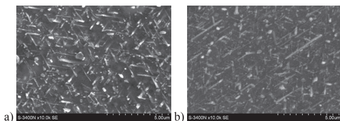
Fig. 11. SEM micrographs of Mg-5Si-7Sn (a) and Mg-5Si-7Sn-2Al (b) alloys aged at 250°C for 148 h with the precipitates of Mg_2Sn phase
