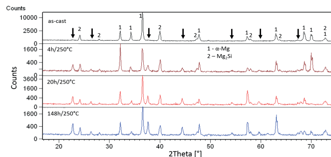
Fig. 8. X-ray diffraction patterns of Mg-5Si-7Sn alloy aged at 250^\circ C
