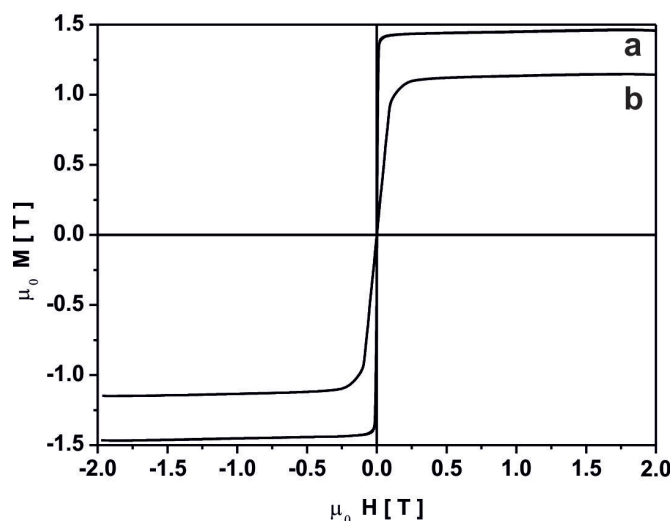
Fig. 8. The static magnetic hysteresis loops, recorded for the samples of the investigated alloy: (a) ribbon, (b) plate
