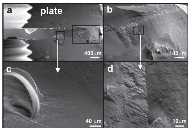
Fig. 6. (a) The SEM image of the plate-shaped sample breakthrough and (b, c and d) the magnifications of the indicated areas
