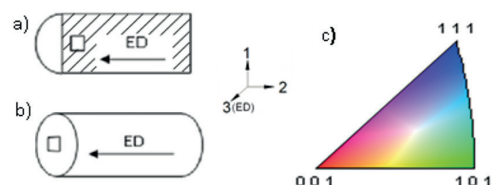
Fig. 1. Indication of sample preparation from longitudinal (1-3) a) and transverse (1-2) b) sections in the extruded billet with marked extrusion direction 3 (ED). c) Inverse pole figure (IPF) for the axis ED
