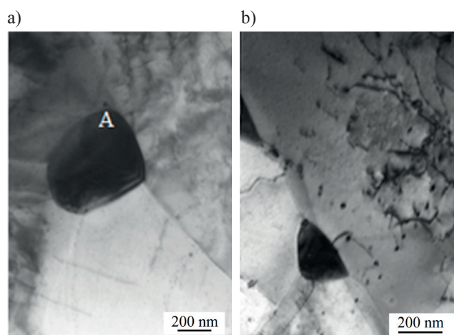
Fig. 10. TEM JEOL JEM 2000FX. Microstructure of 10MnVNb6 steel aged at 690°C for 0.5h after rolling (a, b); (). Plate thickness – 8 mm
