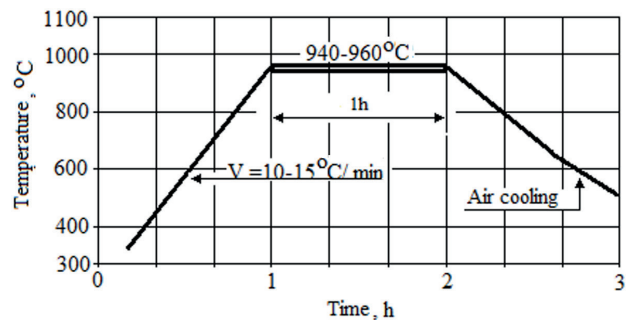
Fig. 2. Technological parameters of normalization of 10MnVNb6 steel
