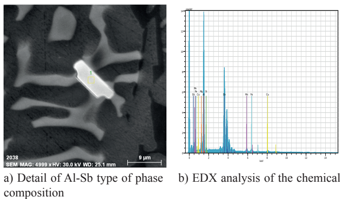
Fig. 13 Sb-based intermetallic phase of alloy 319
