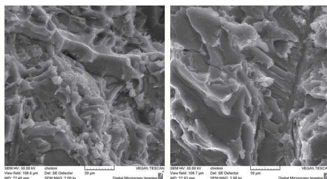
a) detail of the Cu based phase b) detail of the Fe based phase
