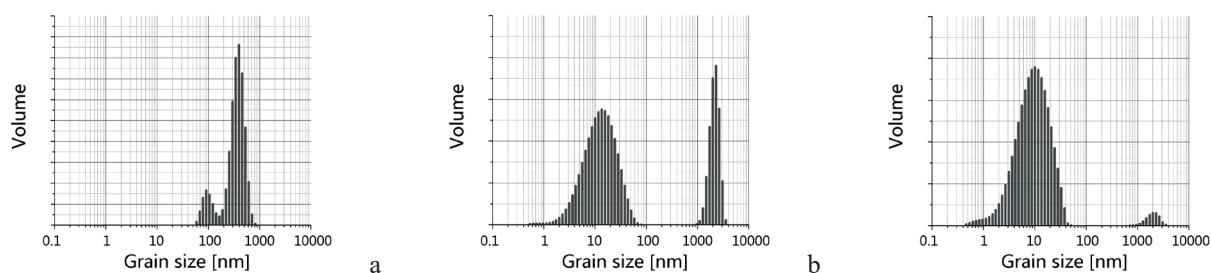
Fig. 3. Grain size distribution of the fillers: a) reference bentonite (BE), b) OBE-1 organophilised bentonite and c) OBE-2 organophilised bentonite
