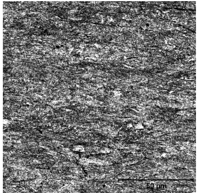
Fig. 9. Material tempered at the temperature 400°C, subjected to cold working treatments, visible 40% material reduction. SEM
