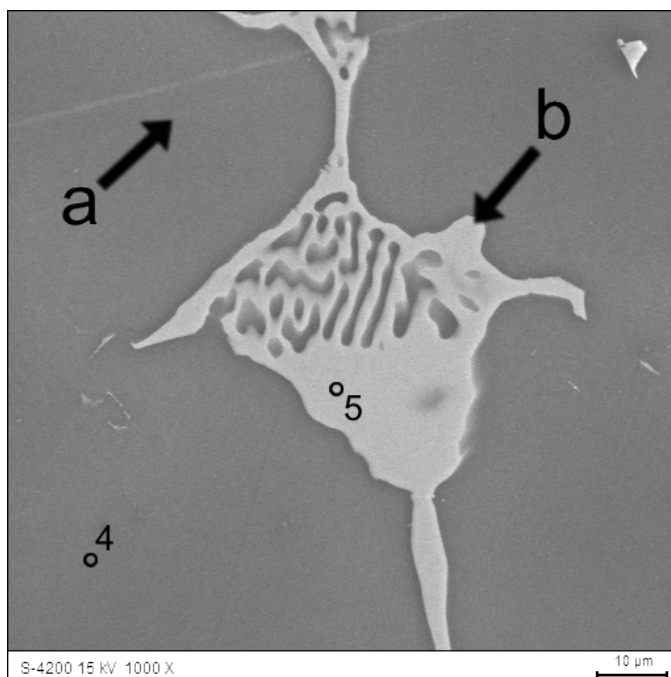
Fig. 5. SEM micrograph of the eutectic compound in WE43 matrix composite reinforced with non-coated 3D textile (1000 \times )
