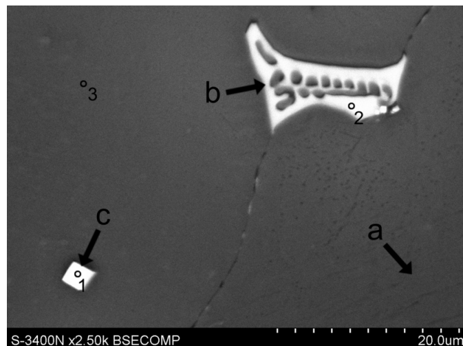
Fig. 1. SEM micrograph of non-reinforced WE43 alloy (2500 \times )
