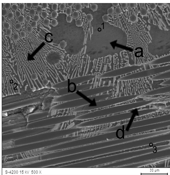
Fig. 3. SEM micrograph of WE43 magnesium matrix composite reinforced with nickel-coated plain textile (500 \times )
