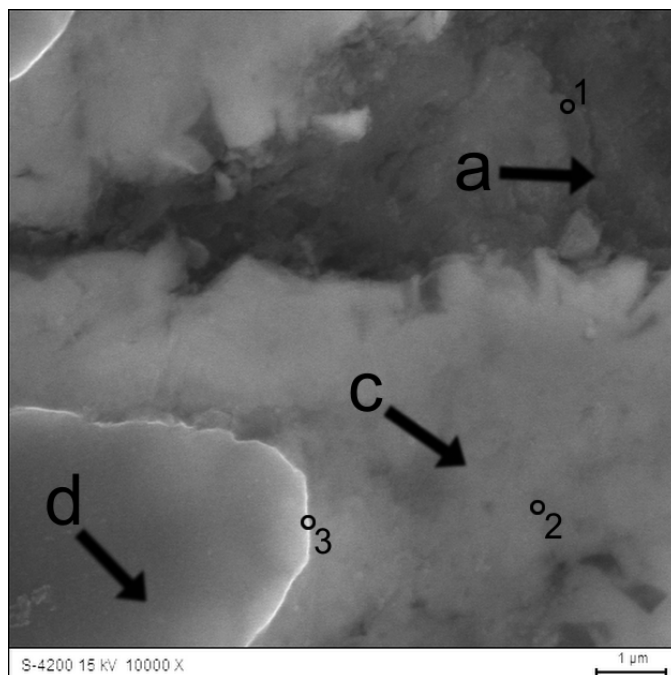
Fig. 4. SEM micrograph of matrix-reinforcement intermediate layer in WE43 matrix composite reinforced with non-coated 3D textile (10000 \times )
