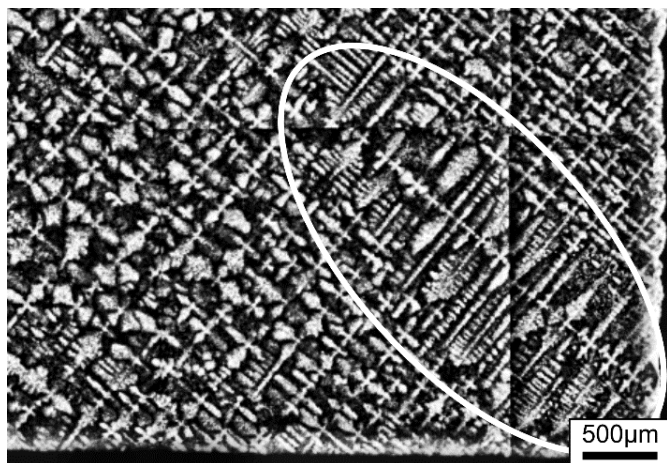
Fig. 8. SEM micrograph (BSE technique) of the blade root dendritic structure in area 4 (Fig. 3)
