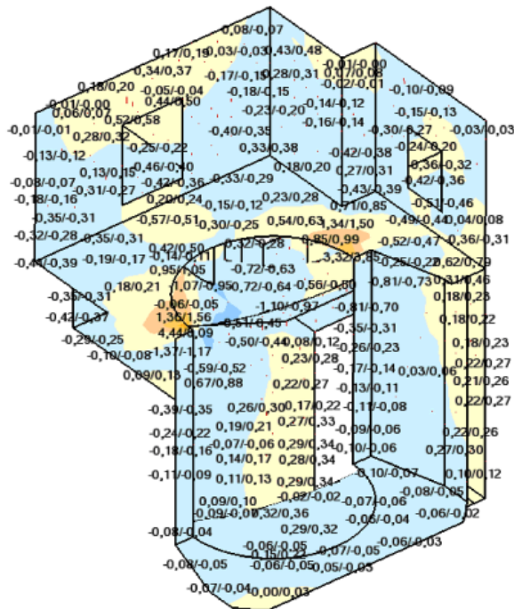
Fig. 7. Map of the reduced normal stress [MPa] occurring in the collar – a view from the side of the shaft
