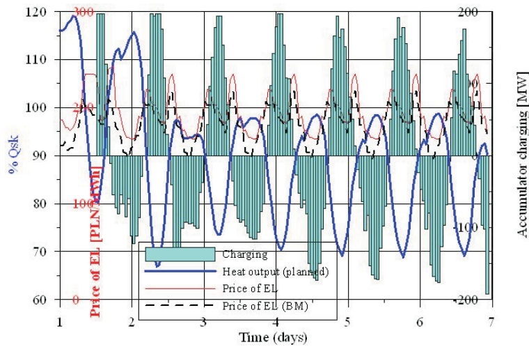
Figure 9. Result of optimisation carried out by the advisory system for 7 days' time.
