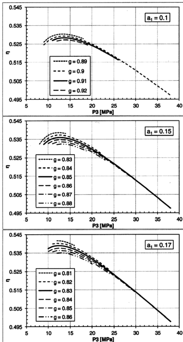
Figure 11. The efficiency, \eta , of the transcritical \text{CO}_2 cycle version No. 2 working with the turbine input pressure p_1 = 40 MPa and temperature T_1 = 700 °C, calculated as a function of interstage pressure p_3 for selected values of the flow fractions a_1 and g .
