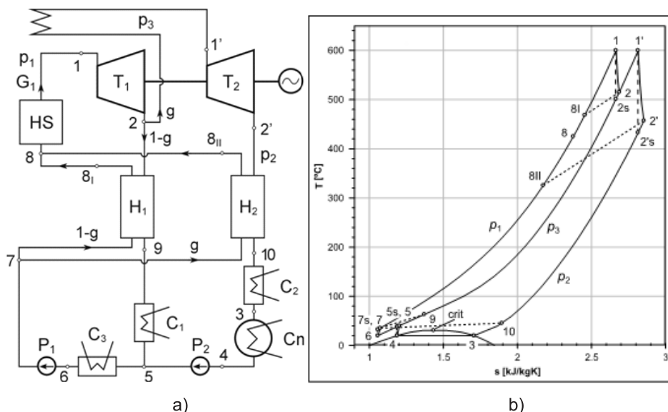
Figure 3. Transcritical CO 2 power cycle, version No. 1: a) schematic view, b) T - s diagram with the cycle principal state points marked. Designations: HS – heat source, T – turbine, H – regenerative heater, C – cooler, Cn – condenser, P – pump.
