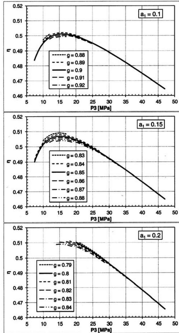
Figure 12. The efficiency, \eta , of the transcritical \text{CO}_2 cycle version No. 2 working with the turbine input pressure p_1 = 50 MPa and temperature T_1 = 600 °C, calculated as a function of interstage pressure p_3 for selected values of flow fractions a_1 and g .
