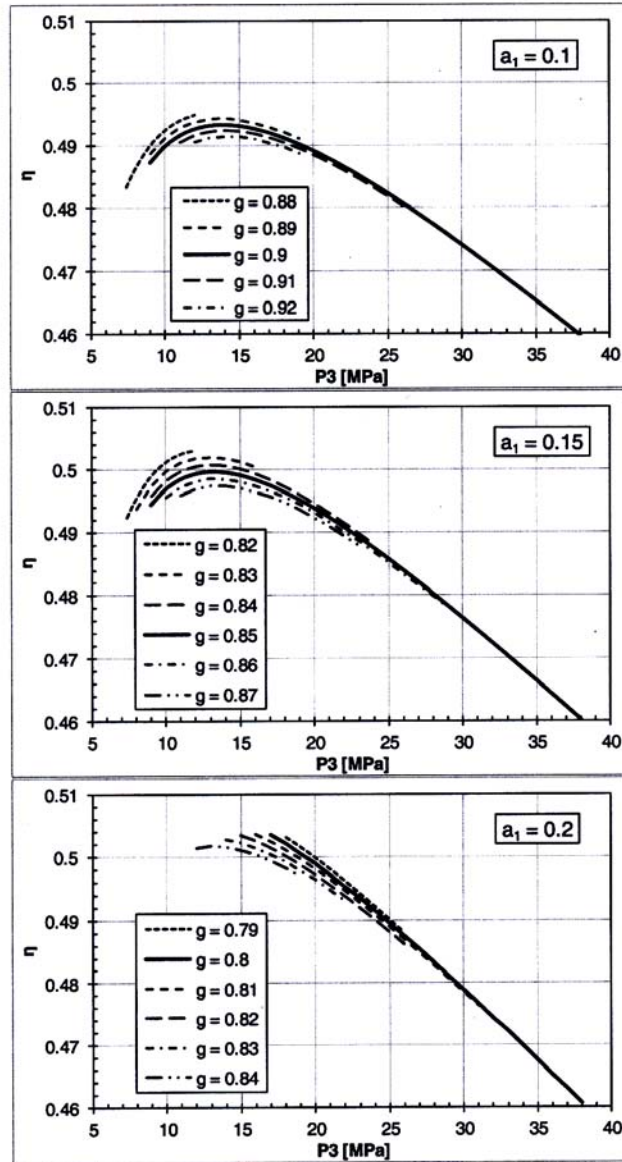
Figure 10. The efficiency, \eta , of the transcritical \text{CO}_2 cycle version No. 2 working with the turbine input pressure p_1 = 40 MPa and temperature T_1 = 600 °C, calculated as a function of interstage pressure p_3 for selected values of the flow fractions a_1 and g .
