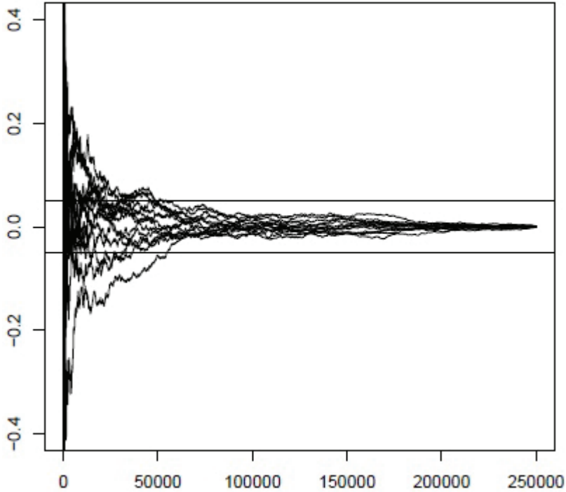
Figure 2. The convergence of CUSUM statistics for the MH algorithm
