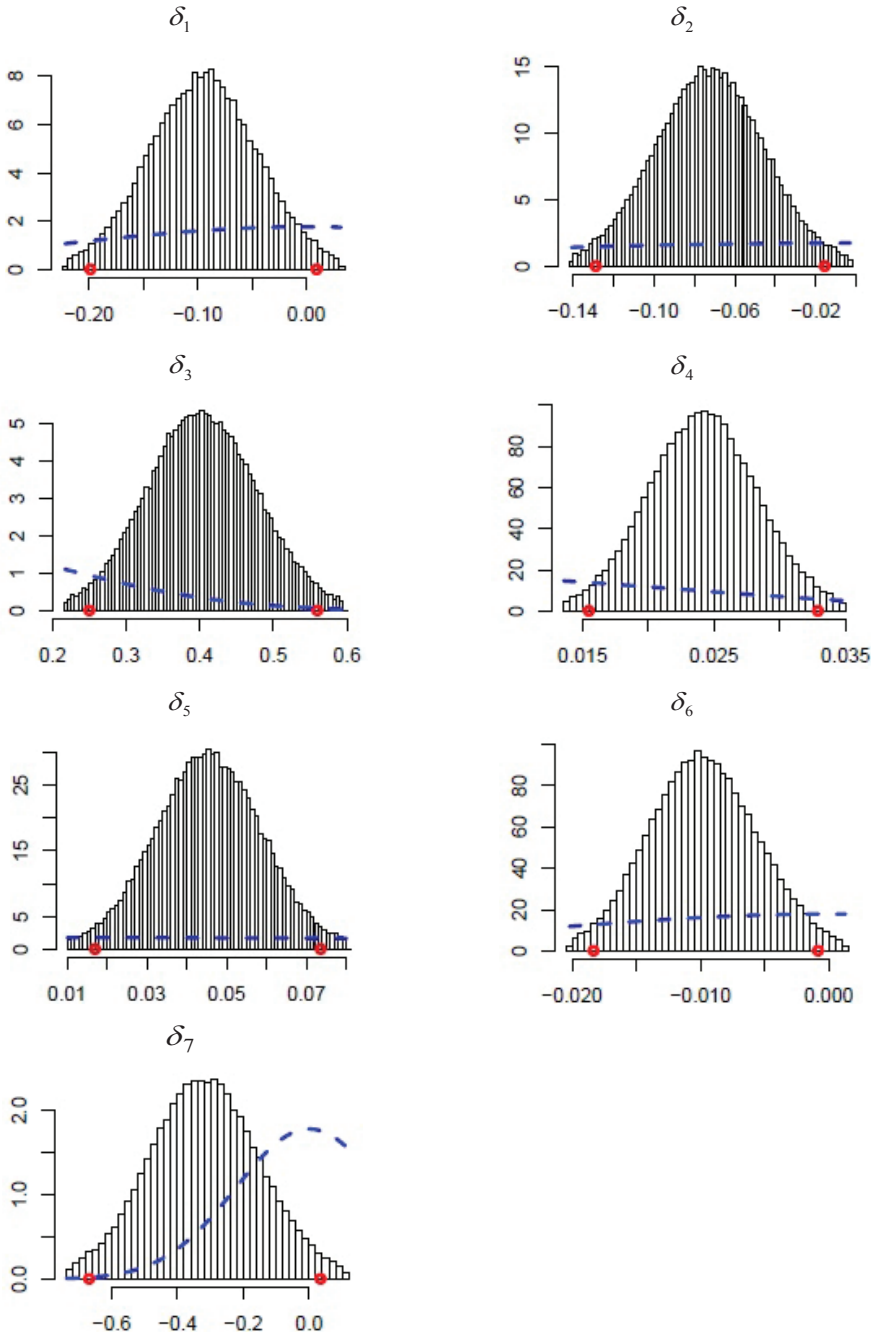
Figure 6. The marginal posterior distributions – the count model
