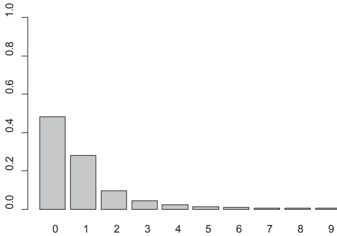
Figure 4. The prior distribution of number of children for a chosen woman
