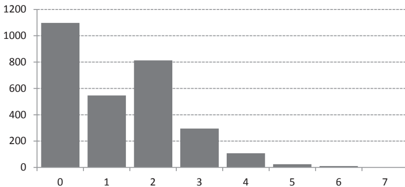
Figure 1. Number of children ever born
