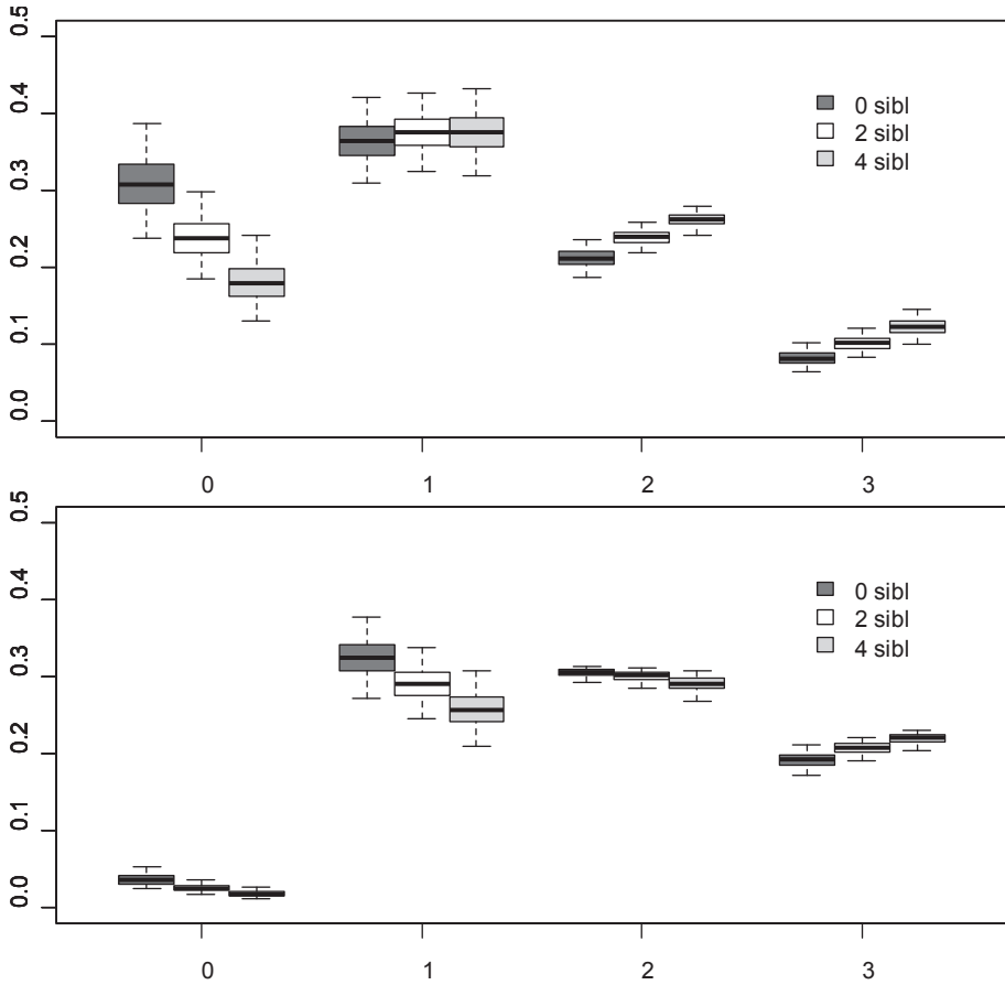
Figure 7. The posterior probabilities of particular number of children for a different number of siblings
