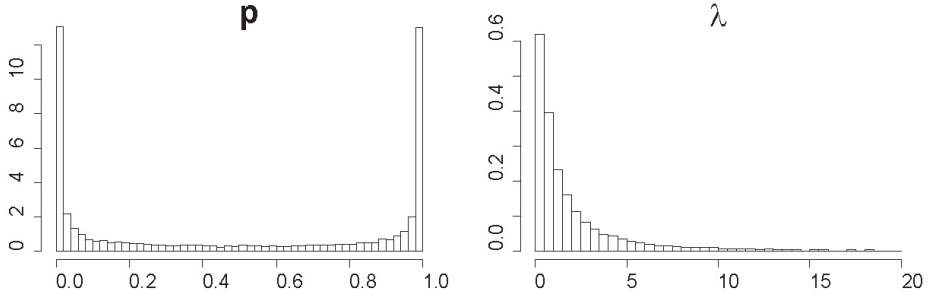
Figure 3. The p and \lambda distributions for a chosen woman
