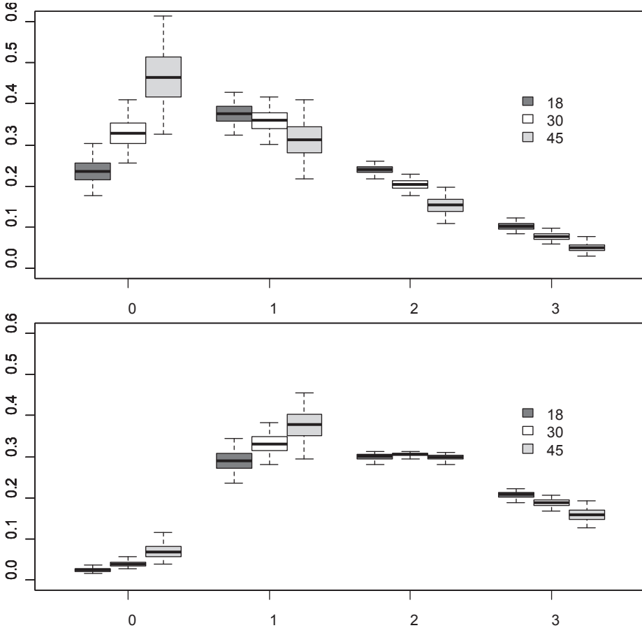
Figure 8. The posterior probabilities of particular number of children for a different mother's age at respondent's birth
