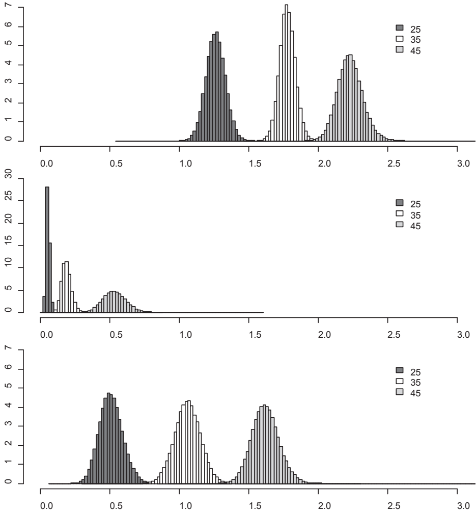
Figure 10. The posterior distributions of expected number of children for type C, D and E
