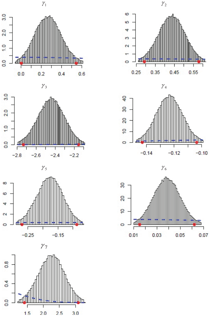
Figure 5. The marginal posterior distributions – the zero model
