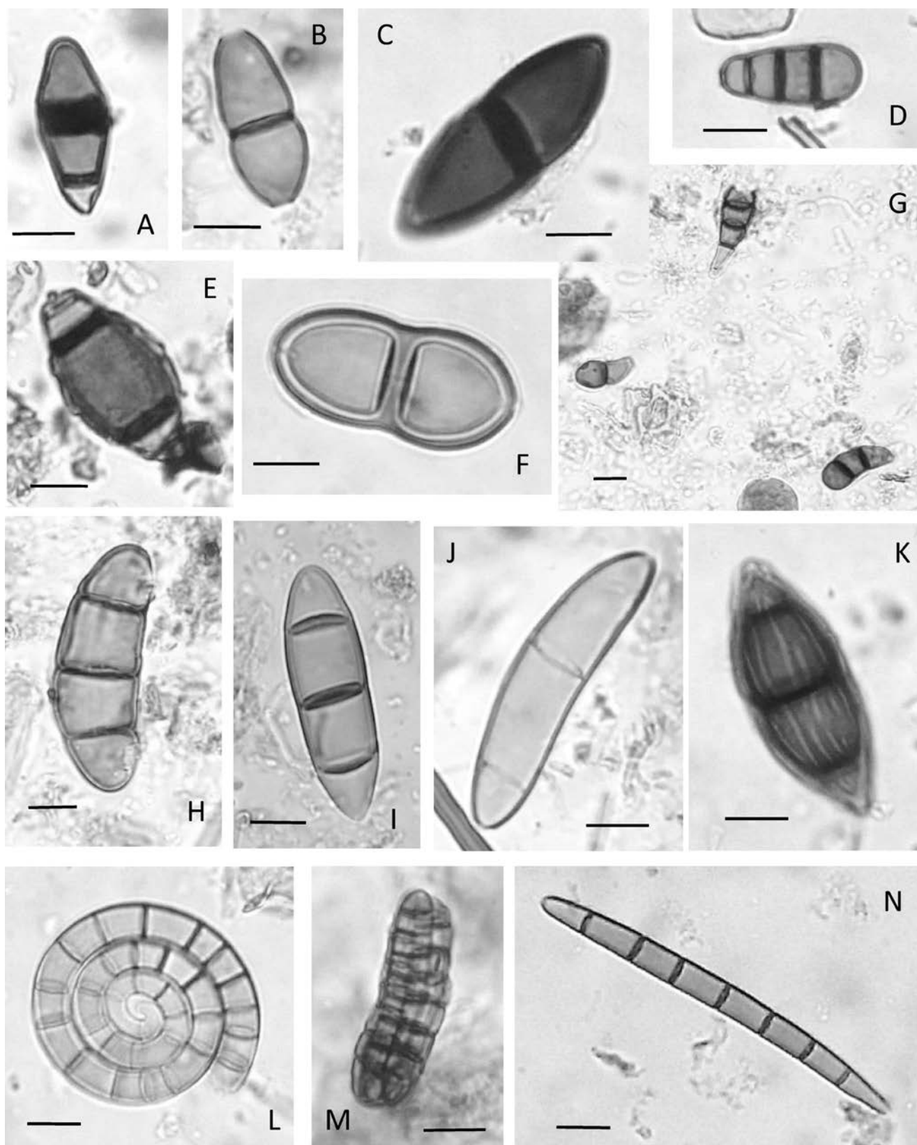
Fig. 6. A BM-2 (96 cm), B HdV 83 (14 cm), C Delitschia sp. (84 cm), D Brachysporium bloxami (84 cm), E Brachysporium pendulisporum (96 cm), F Puccinia -type (38 cm), G HdV 10 (4 cm), H Meliola ellisii (4 cm), I HdV 20d (4 cm), J BM-3 (32 cm), K HdV 463 (108 cm), L Helicoon pluriseptatum (52 cm), M Dictiosporium australiense (BM-4) (112 cm), N Geoglossum sphagnophilum (40 cm). Bar scale 10 µm. The indication in cm refers to the position in the core.
