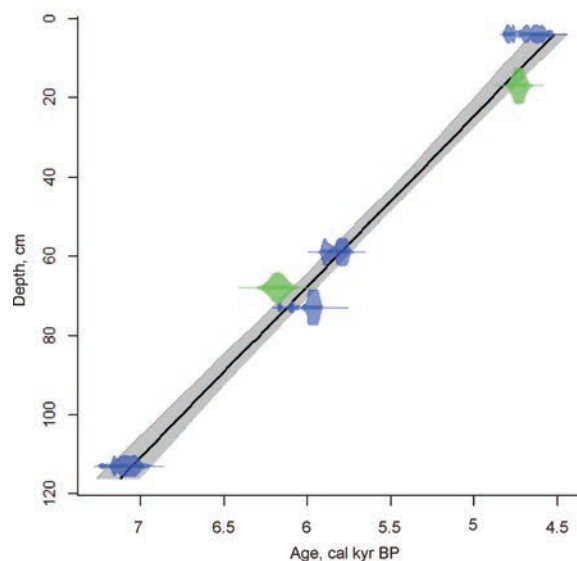
Fig. 2. Age-depth model of the Borsteler Moor based on radiocarbon dating of peat bulk (blue) and dendrochronological dating (green).
