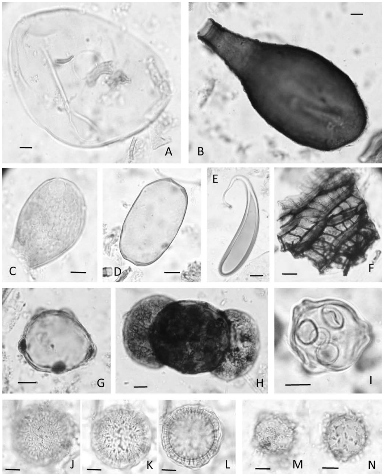
Fig. 4. A Arcella sp. (26 cm), B Habrotrocha angusticolis lorica (20 cm), C Assulina muscorum (16 cm), D Amphitrema flavum (18 cm), E spermatophore of copepods (6 cm), F charred Sphagnum leaves (6 cm), G Carpinus betulus infected by dark-coloured hyphae (4 cm), H Pinus diploxylon -type with inner covered by dark-coloured hyphae (38 cm), I Betula pollen with chytridiomycetes sporangia (96 cm), J–L BM-1 (10 cm), M–N HdV 59 (4 cm). Bar scale 10 µm. The indication in cm refers to the position in the core.
