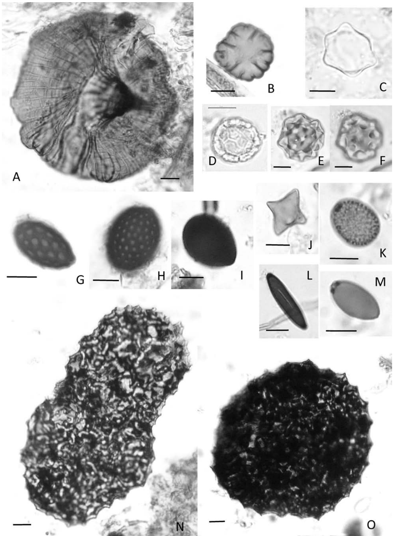
Fig. 5. A Fruiting-body of HdV 8D (56 cm), B HdV 13 Desmidiospora (4 cm), C HdV 66 cf. Inocybe sp. (6 cm), D Bryophytomyces sphagni (50 cm), E–F HdV 724 (30 cm), G Gelasinospora retispora (6 cm), H Gelasinospora sp. (4 cm), I Acrogenospora sphaerocephala (112 cm), J HdV 365 cf. Inocybe sp. (104 cm), K HdV 733 (10 cm), L Ustulina deusta (26 cm), M Podospora sp. (30 cm), N–O zygospores of Mucor sp. (BM-5) (38 and 30 cm, respectively). Bar scale 10 \mu m. The indication in cm refers to the position in the core.
