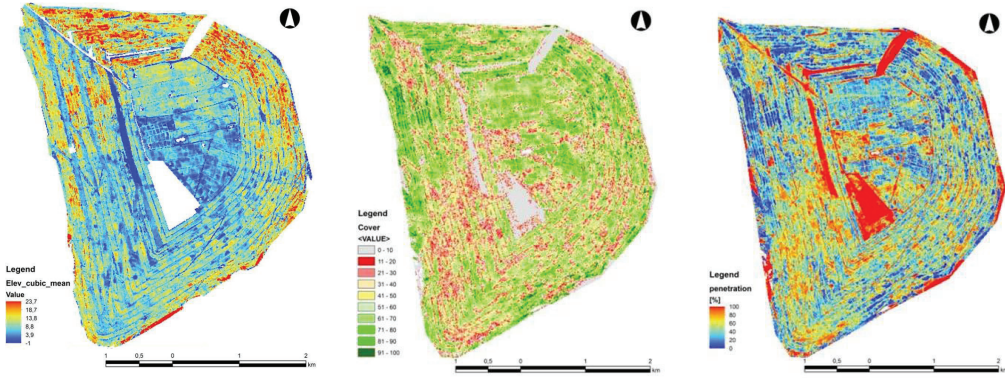
Fig. 7. The Belchatow spoil heap – 3D matrix, from left: height of vegetation, cover density and penetration
